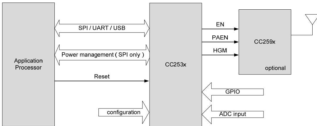
Figure 1 CC2530 Interface
